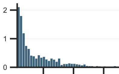
m4: DoG+HRF
