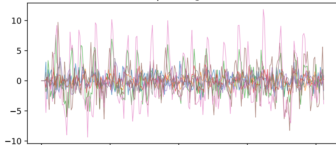
Cleaned BOLD | M1-signal voxels (n=8)
