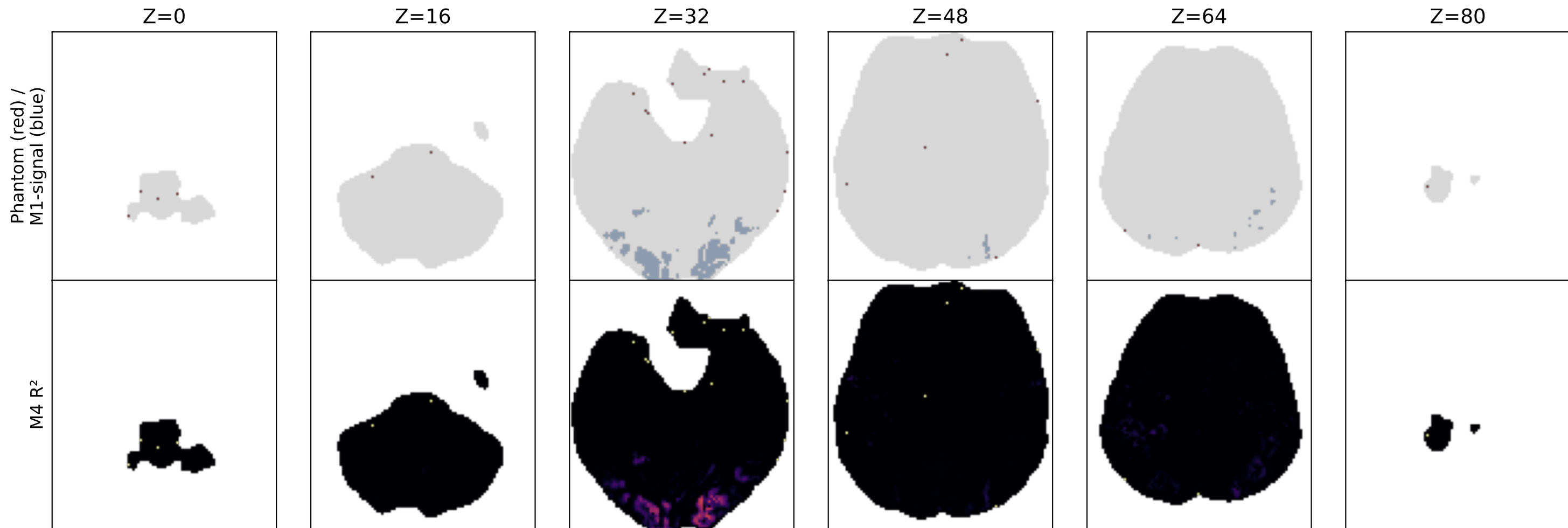
Sub-05 | Spatial: phantom voxels (red), M1-signal (blue), and M4 R 2 (bottom)
