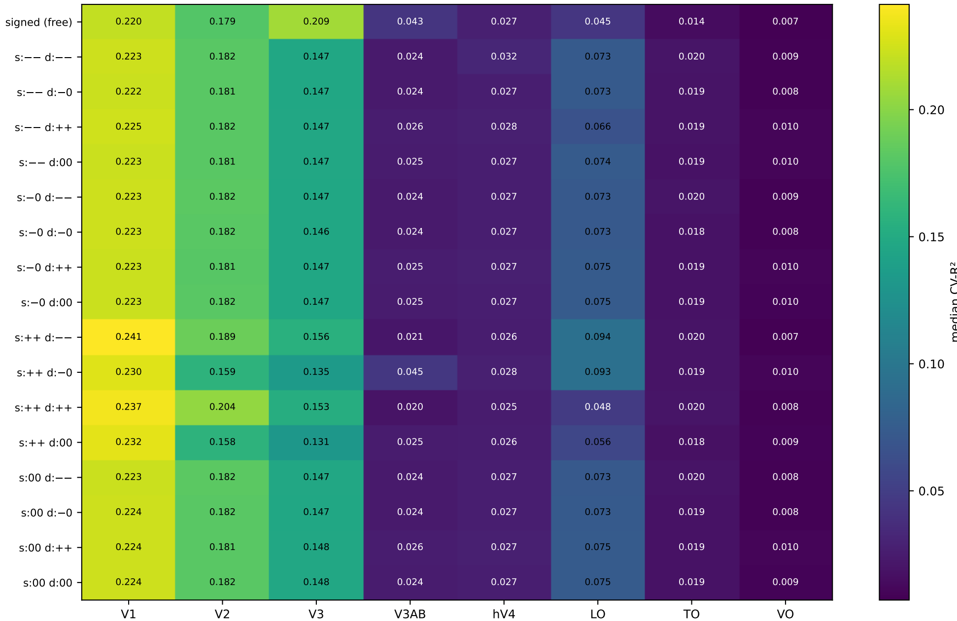
CV-R 2 heatmap: class × ROI (median across subjects, n_fits=3508)
