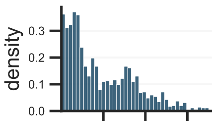
m5: DN
