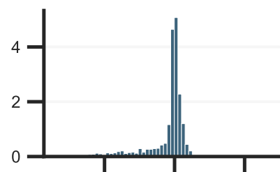
m6: DN+HRF
