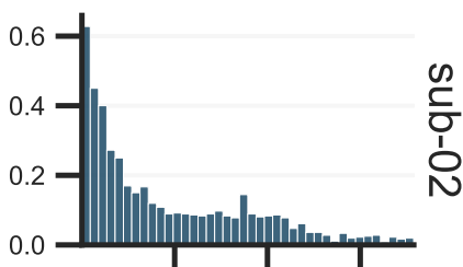
m6: DN+HRF
