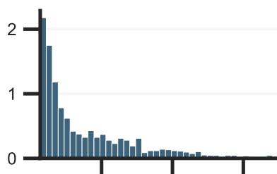
m4: DoG+HRF
