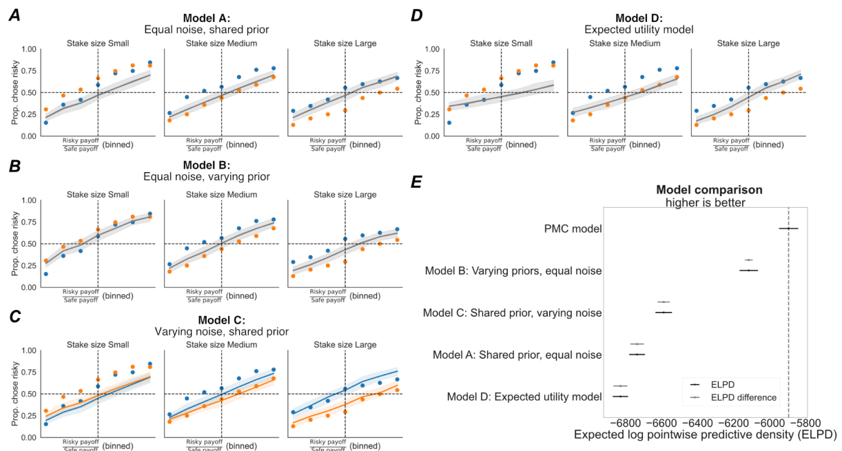
Figure 3: A-D) Posterior predictive plots for alternative models of different complexity. Unlike the PMCM, none of the tested models can explain all qualitative patterns in the
