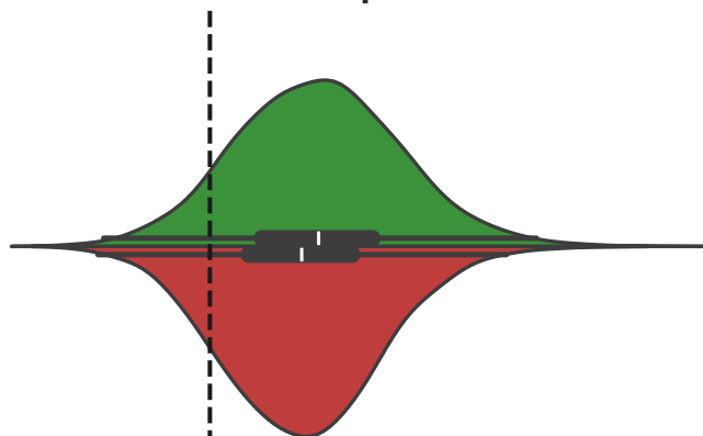
Indifference point
