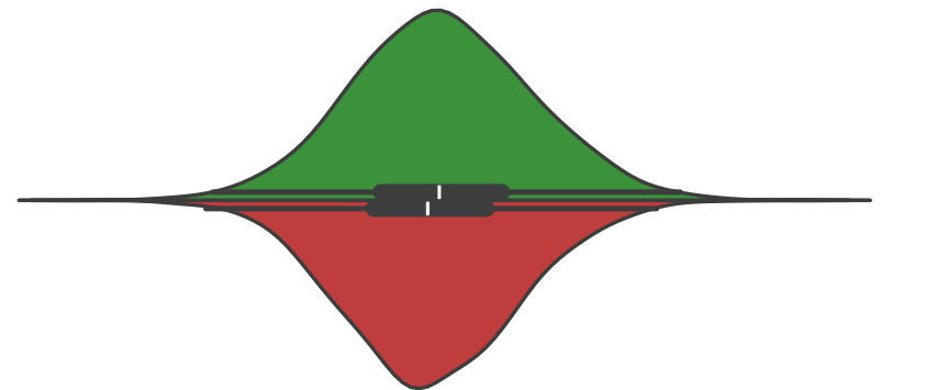
Psychometric slope
