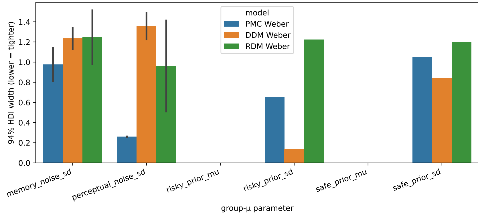
HDI tightening: PMC vs DDM vs RDM on the Weber 'TMS-on-both' fits (shared cognitive front-end, different likelihoods)
