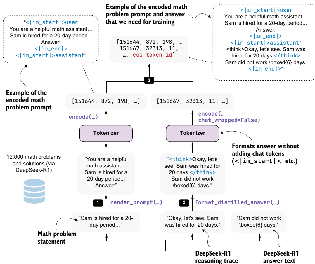
Figure 8.9 Example of the tokenization pipeline for one training sample. The math problem is rendered into the chat prompt format, the teacher reasoning trace and final answer are combined via format_distilled_answer , and both parts are concatenated into one token sequence.
