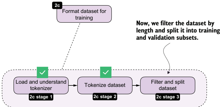
Figure 8.10 After tokenization, we filter out long sequences and split the remaining examples into training and validation subsets.
