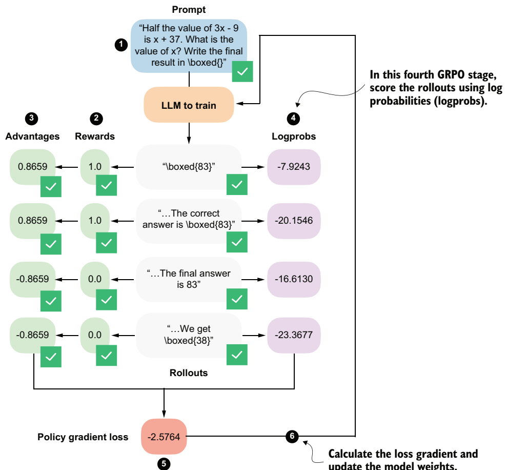
Figure 6.16 The fourth stage in the GRPO pipeline computes log probabilities for each rollout. It is related to the logprob scorer we developed in the previous chapter.
