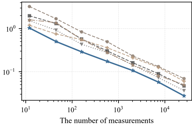
Dense four-qubit ensemble
