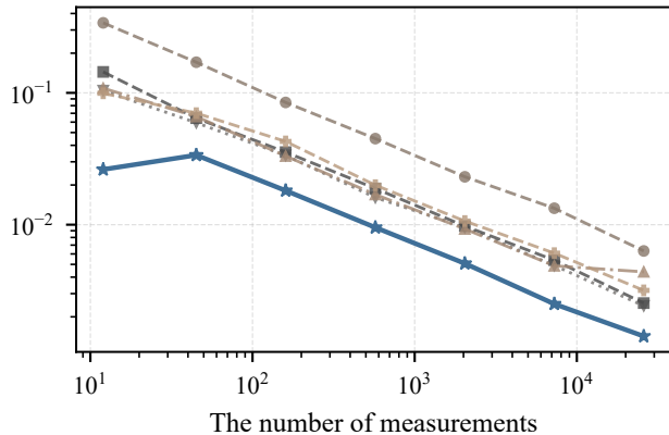
Sparse four-qubit ensemble
