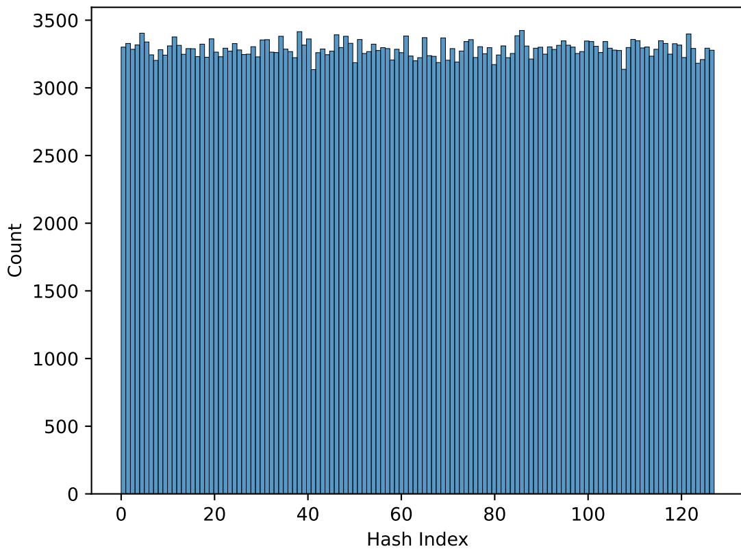
Hash Distribution
