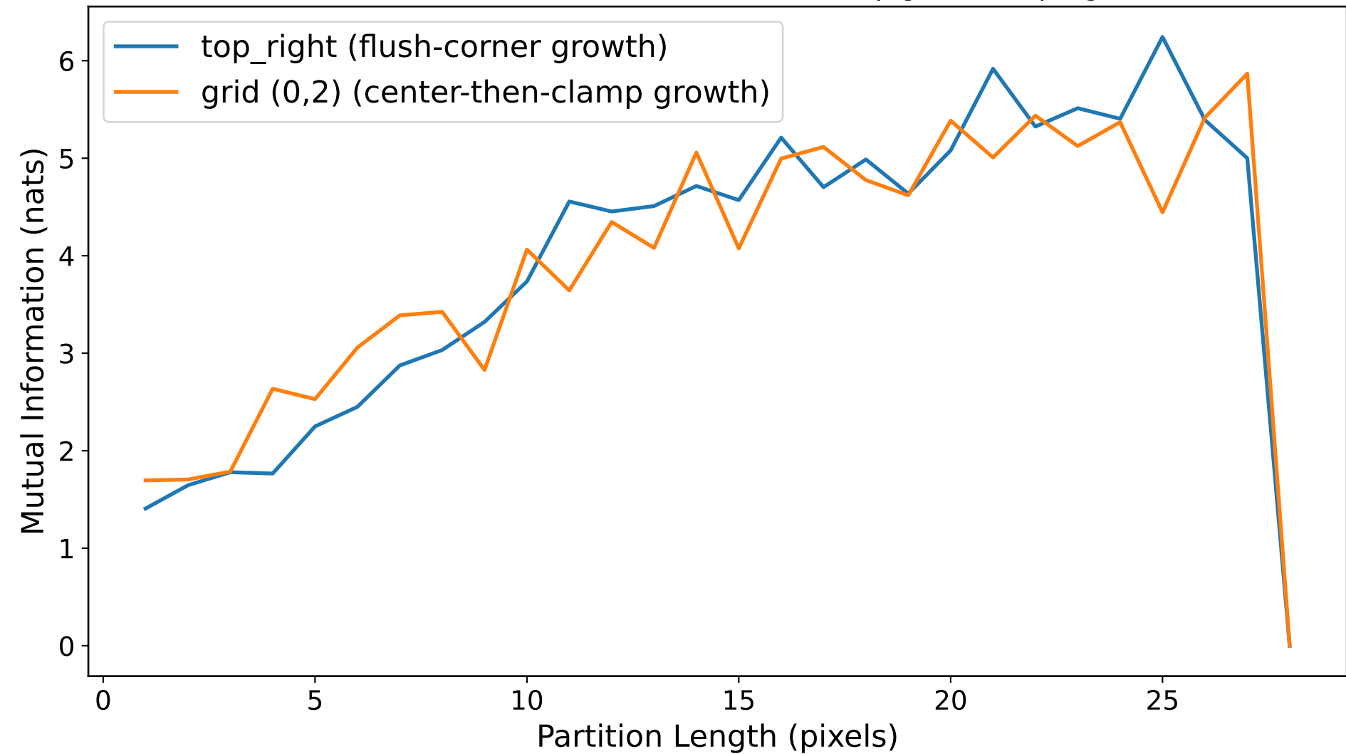
CIFAR-10: flush-corner vs. center-then-clamp growth (top-right)
