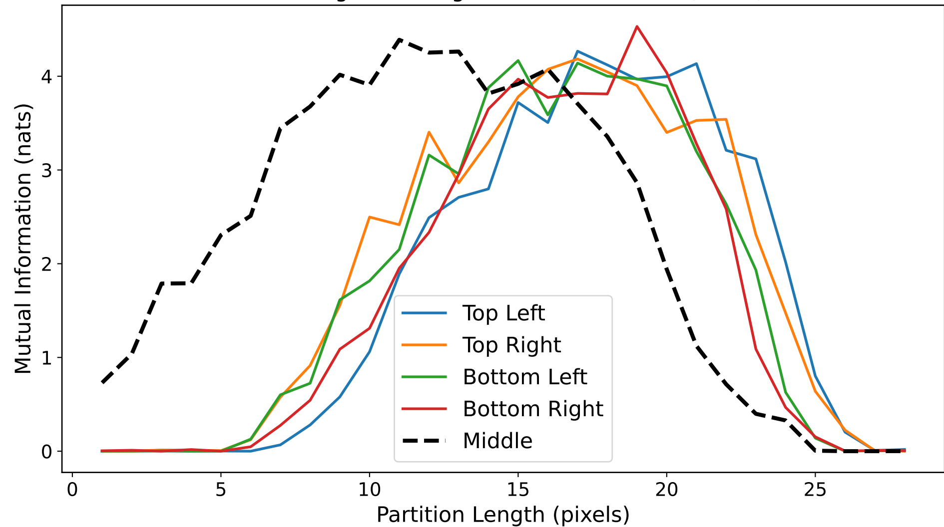
MI scaling from image corners vs. middle (mnist)
