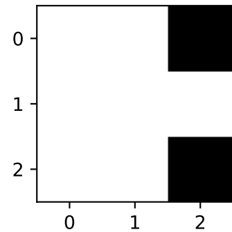
Pixel mask
