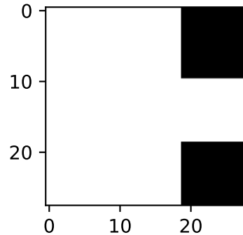
Pixel mask
