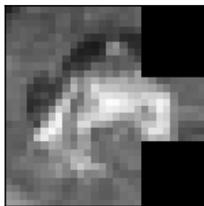
Zero-pruned
