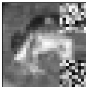
Noise-pruned
