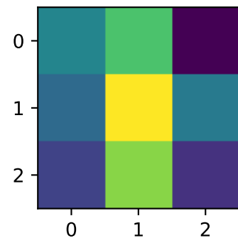
Kept tiles (7/9)
