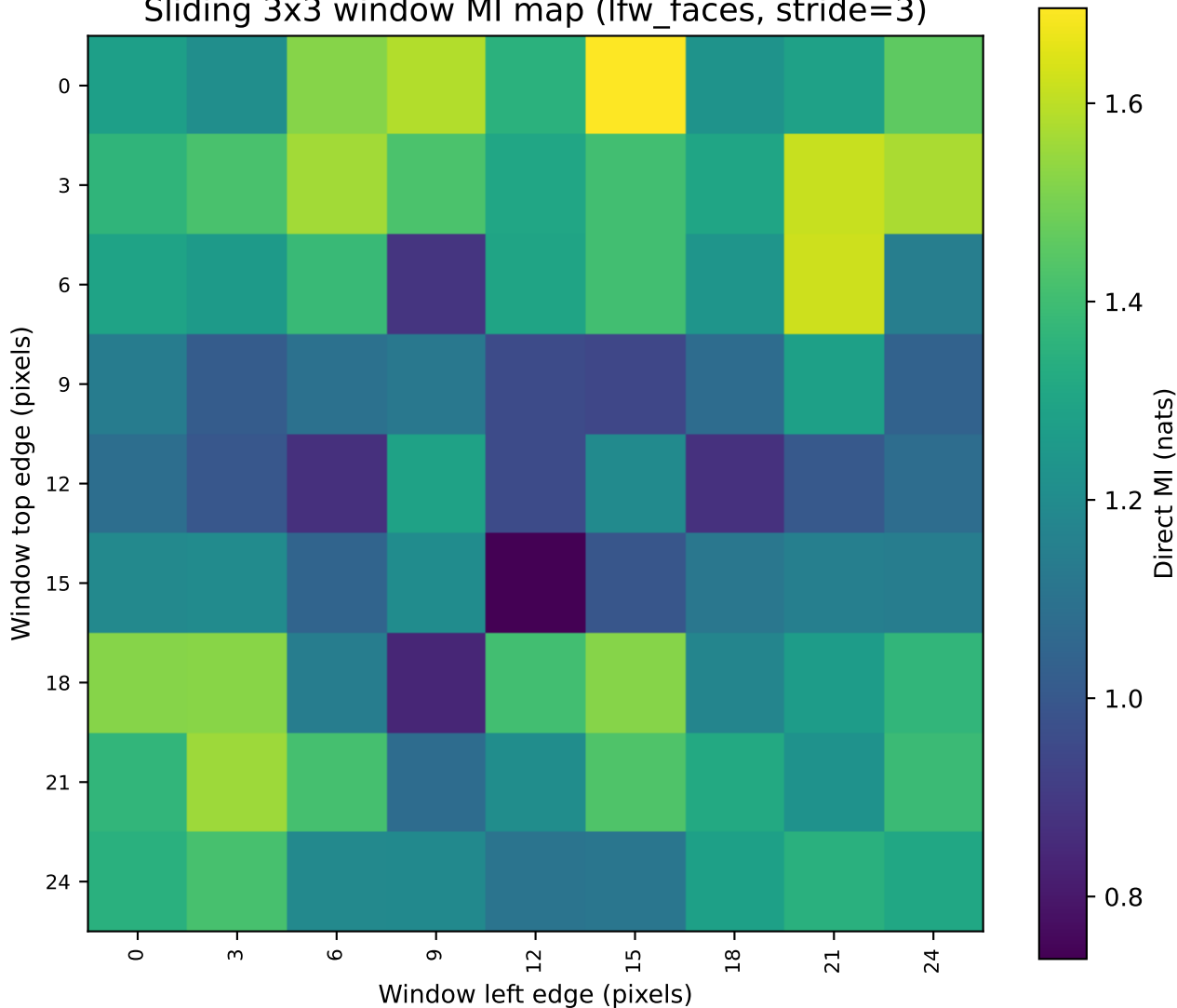
Sliding 3x3 window MI map (lfw_faces, stride=3)
