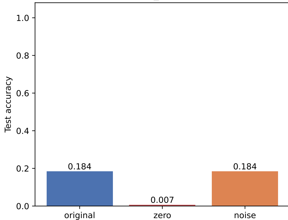
lfw_faces
