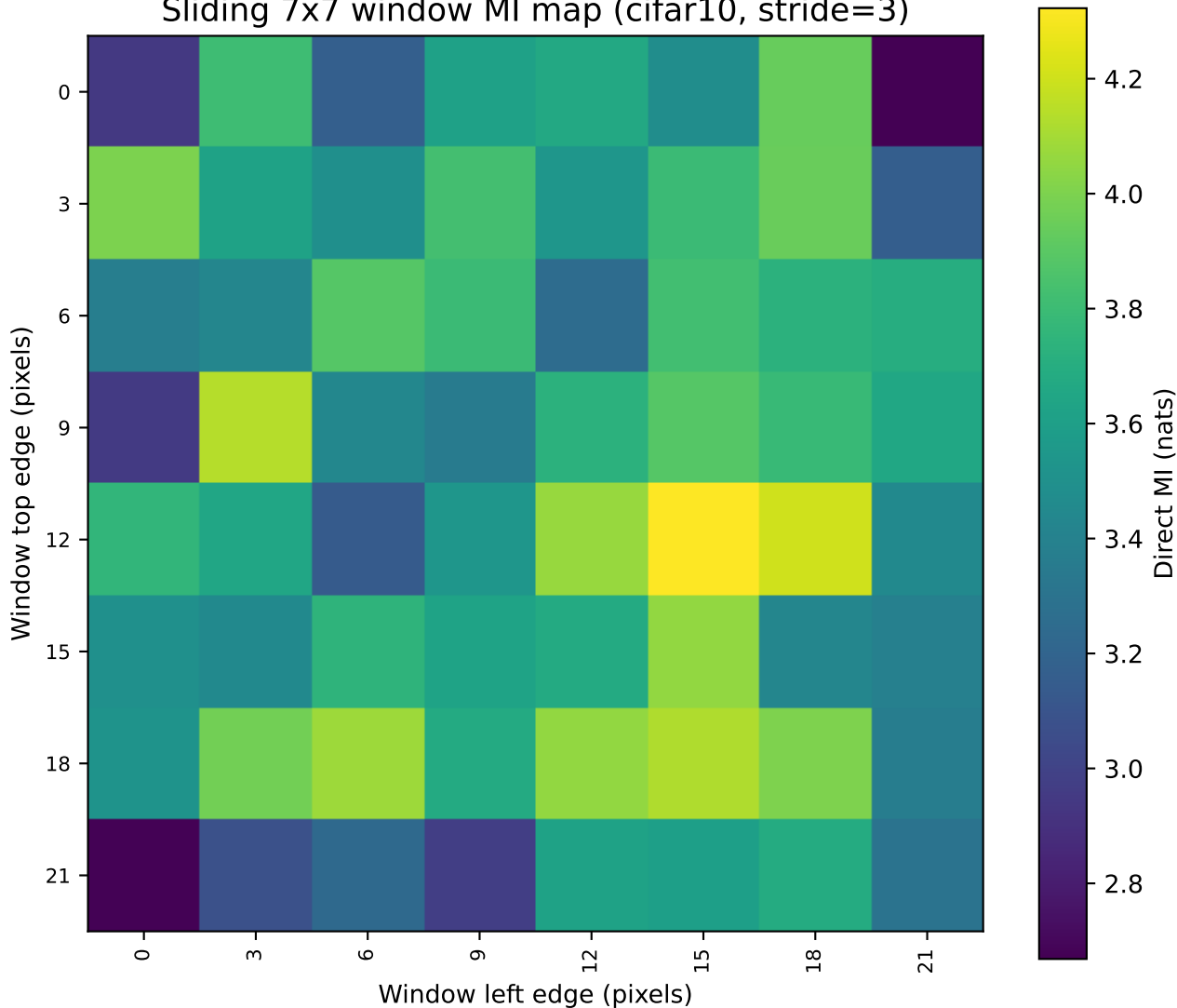
Sliding 7x7 window MI map (cifar10, stride=3)
