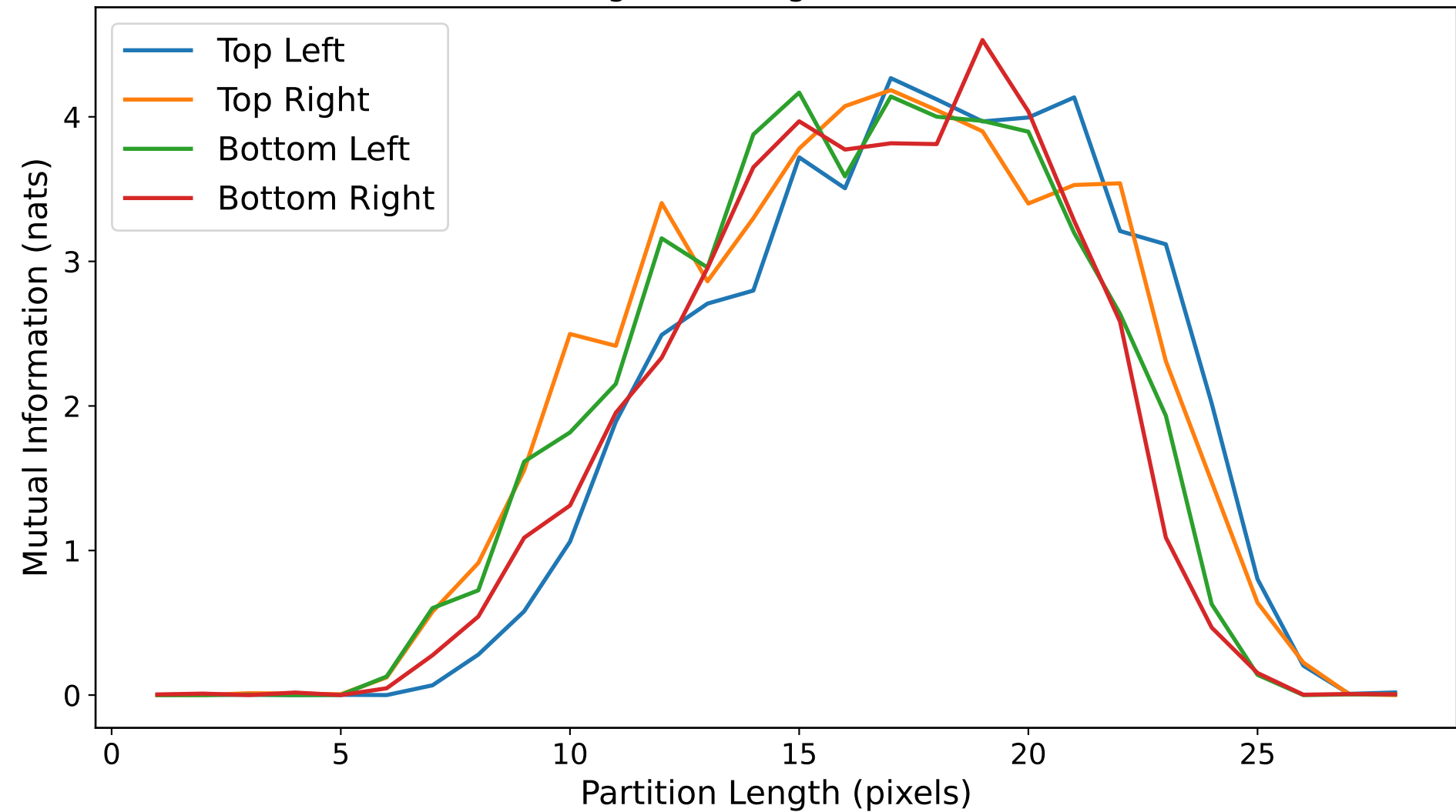
MI scaling from image corners (mnist)
