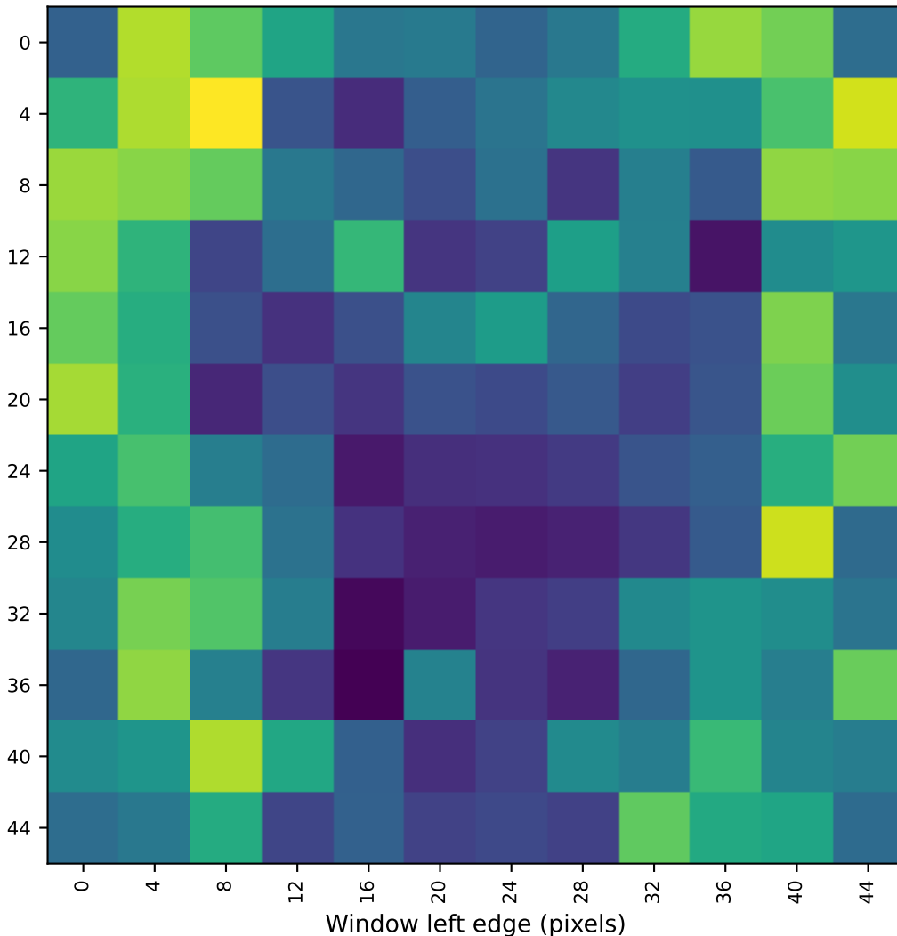
Sliding 4x4 window MI map (fer2013_hf, stride=4)
