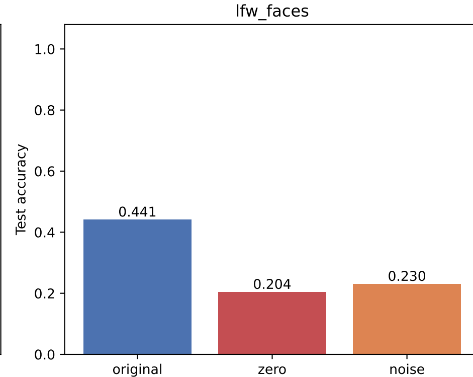
Effect of pruning the lowest-MI 50% of tiles (keep 50%)
