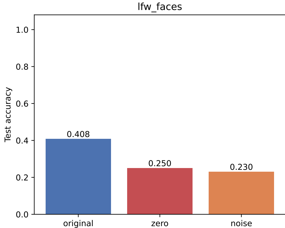
Effect of pruning the lowest-MI 25% of tiles (keep 75%)
