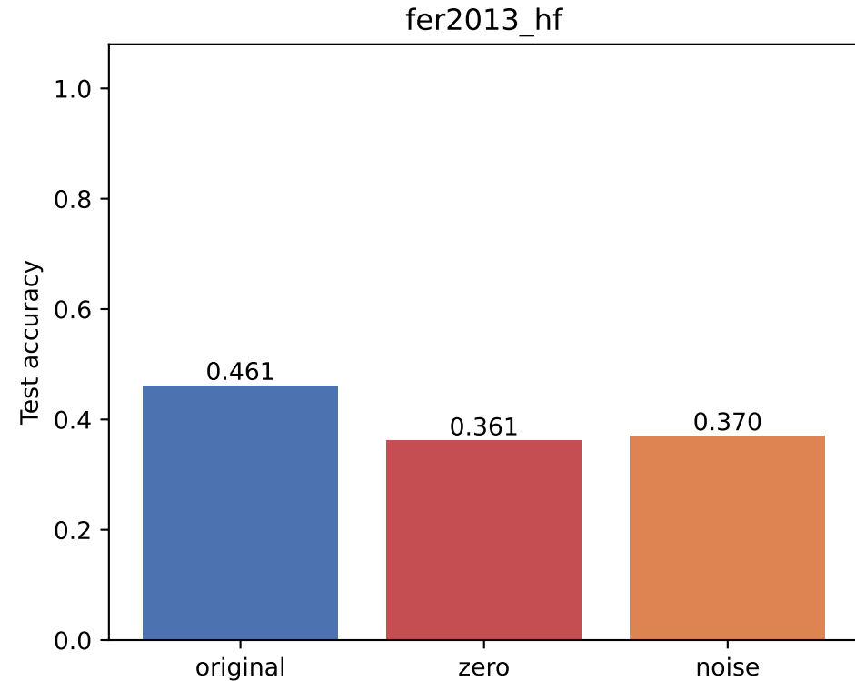
Effect of pruning the lowest-MI 25% of tiles (keep 75%)
