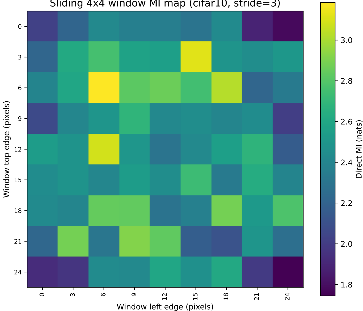
Sliding 4x4 window MI map (cifar10, stride=3)
