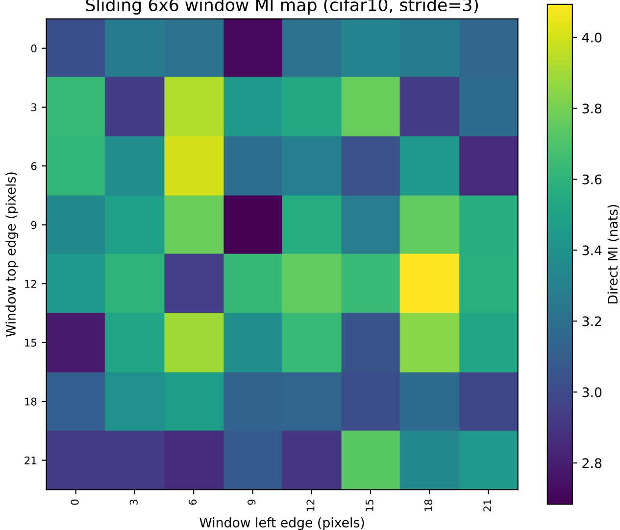
Sliding 6x6 window MI map (cifar10, stride=3)
