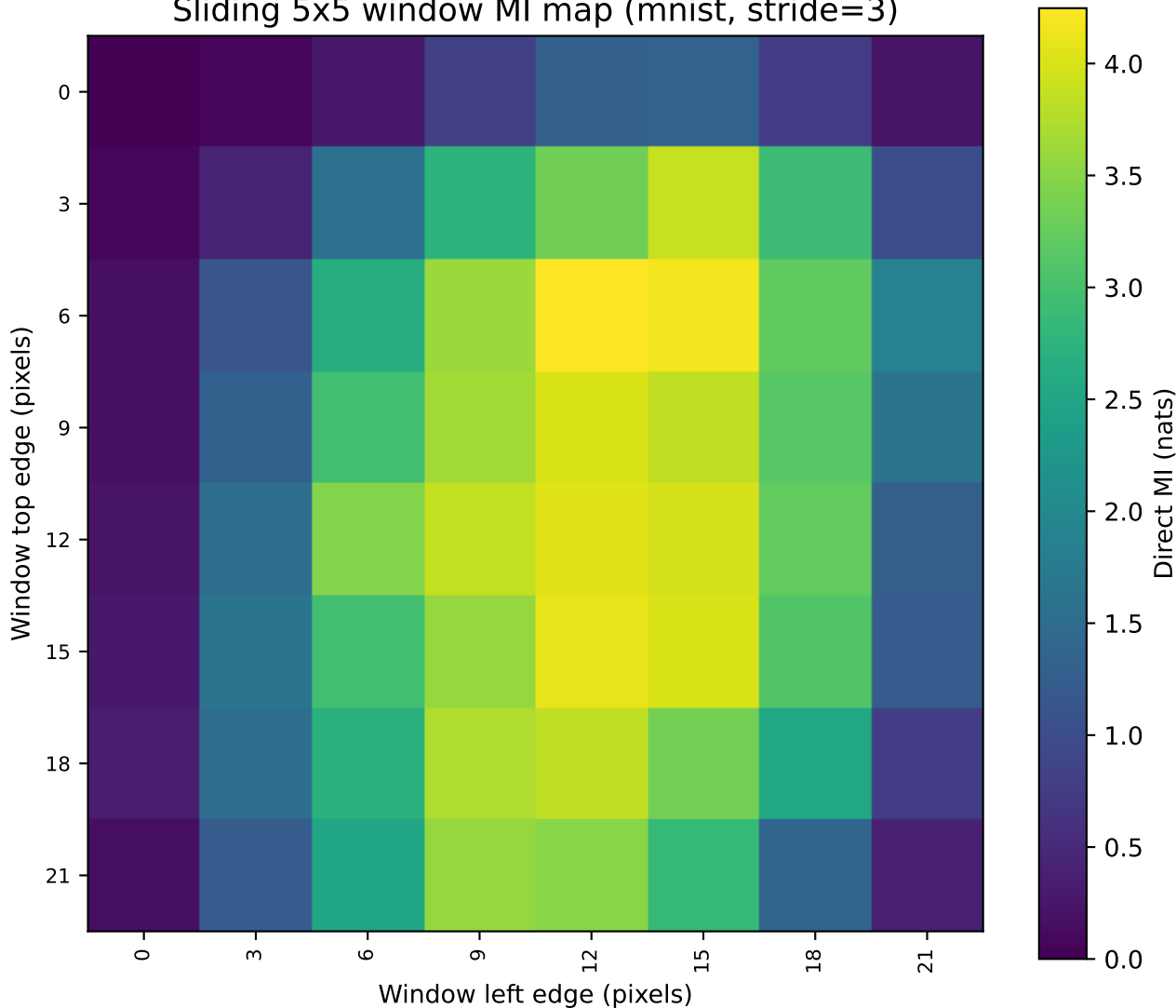
Sliding 5x5 window MI map (mnist, stride=3)
