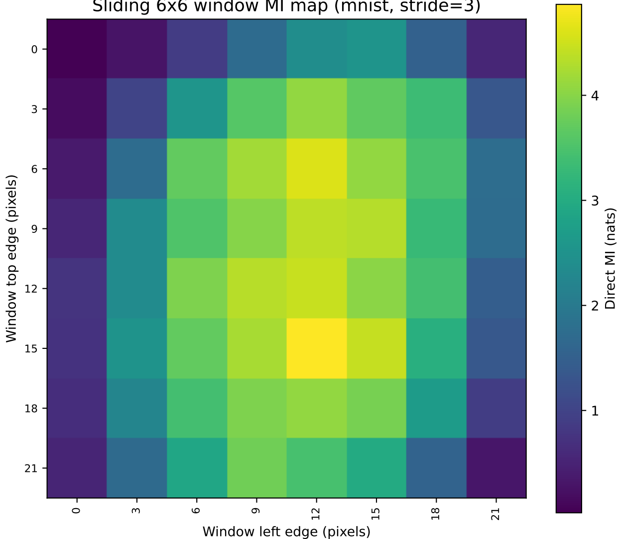
Sliding 6x6 window MI map (mnist, stride=3)
