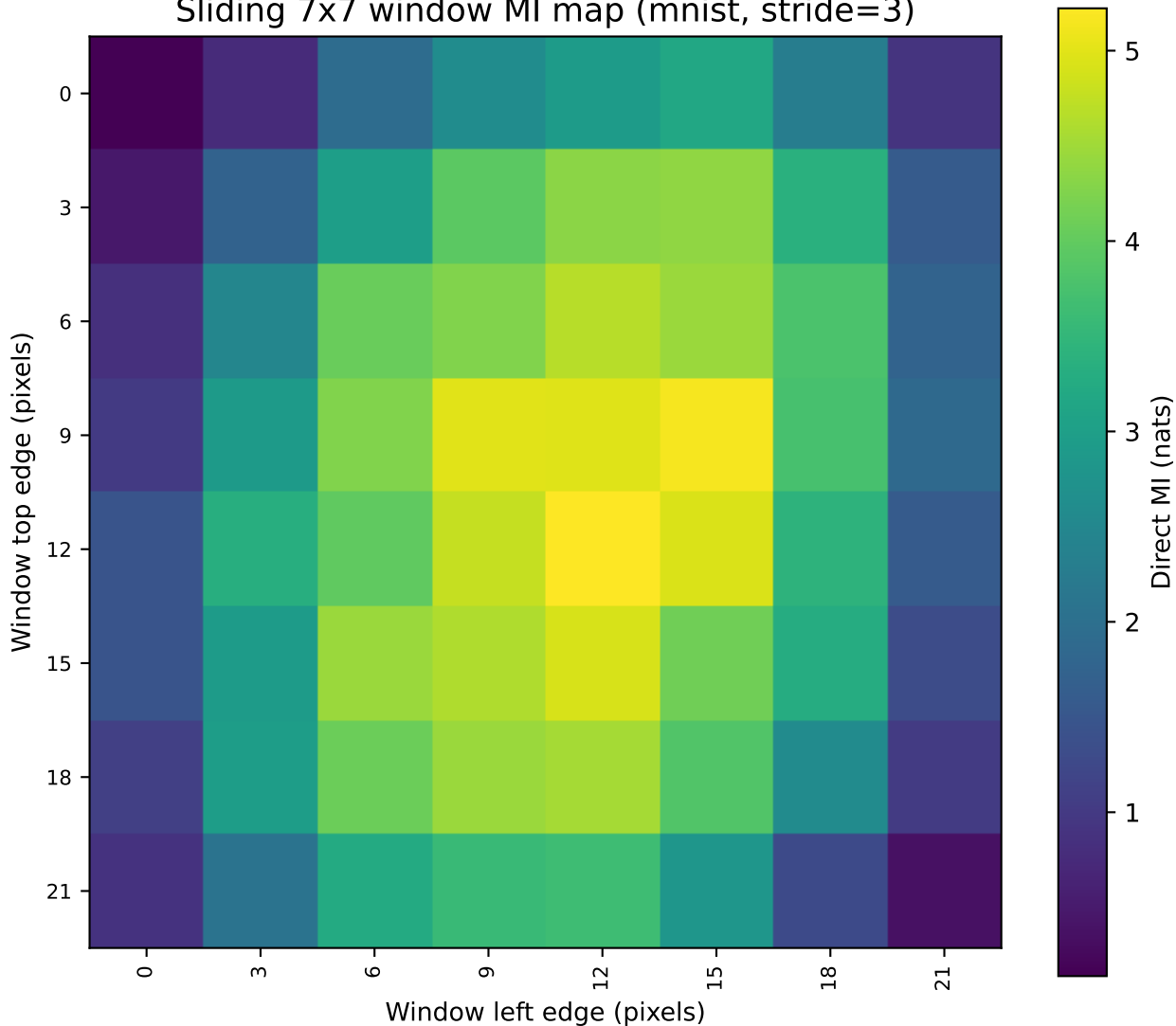
Sliding 7x7 window MI map (mnist, stride=3)
