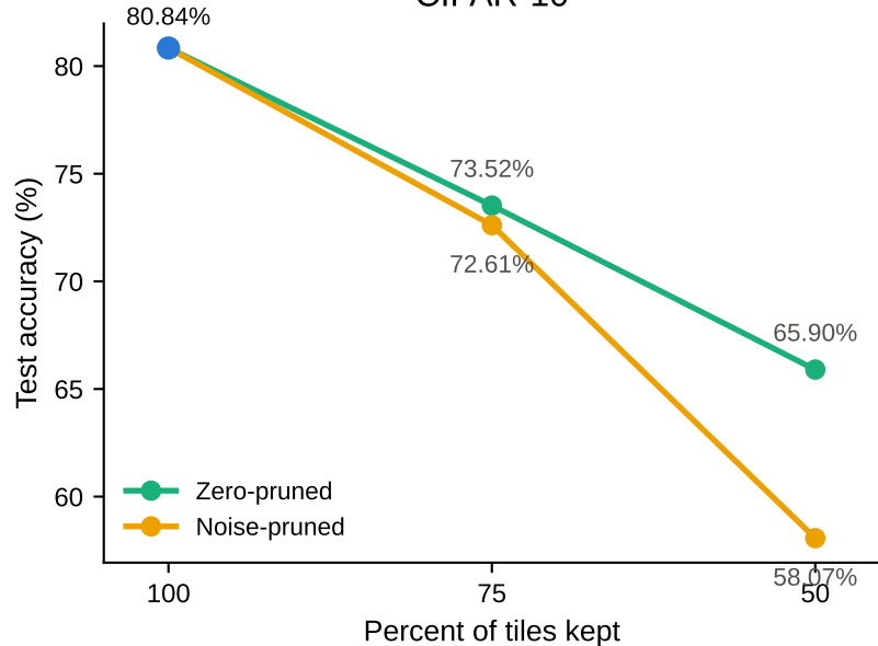
CIFAR-10
