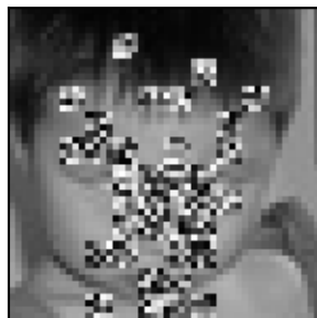
Noise-pruned
