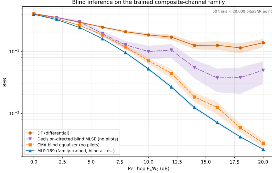
Figure 6.6: No pilots or per-block CSI; fresh realizations from the training family. The evaluated CMA and MLP means are close, while decision-directed MLSE has a non-monotonic high-SNR tail. Historical bands are descriptive; the neural training hierarchy prevents treating all pooled trials as independent confidence evidence. The MLP avoids test-time adaptation but uses family knowledge acquired in training. No claim against all blind equalizers is made
