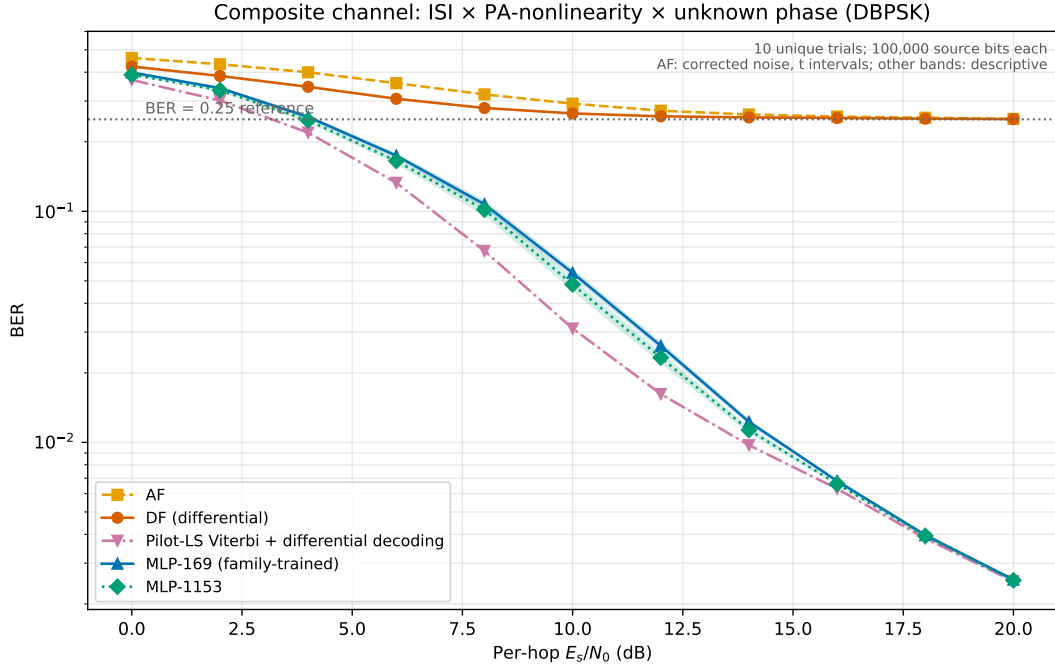
Figure 6.4: Fixed ISI and amplifier with random block phase, DBPSK. The corrected AF curve uses ten unique fixed-budget trials and Student- t intervals. Other curves retain historical point estimates and descriptive bands, which are not calibrated equivalence tests. Both MLPs were trained on this cascade family. Similar high-SNR rounded values do not demonstrate equal BER
