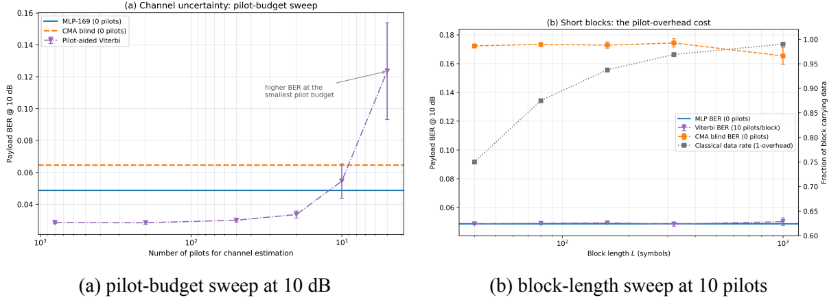
Figure 6.5: Finite-pilot regime; both panels are means over 50 channel draws at 20,000 bits/point. (a) Pilot-aided Viterbi outperforms the pilot-free MLP down to approximately 20 pilots per block, loses its edge by 10 pilots, and collapses at 5 pilots when the least-squares estimate becomes too noisy to construct a reliable trellis ( 0.1235 \pm 0.0304 ); the MLP is flat across the sweep, operating with a family-trained discriminative estimator and requiring no pilots. (b) With 10 pilots per block, pilot-aided Viterbi and the MLP have no detected payload-BER difference at the evaluated block lengths (both \approx 0.049 ), but the classical receiver’s pilot overhead grows from approximately 1% at L = 1000 to 25% at L = 40 . The tested CMA implementation has higher BER throughout. The MLP uses no pilots and has no resolved BER difference from the pilot-aided receiver at this budget; equivalence and superiority to untested pilot-free methods are not established
