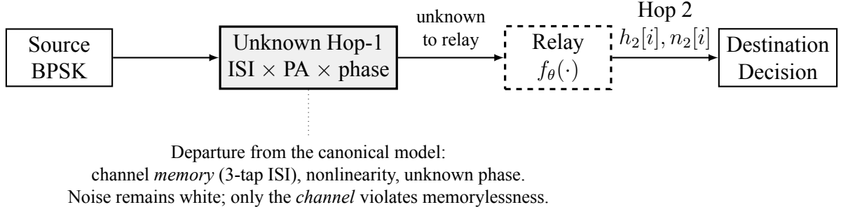
Figure 6.1: Schematic of the composite impairment study. Hop 1 includes memory, amplifier non-linearity, and block phase; Hop 2 is compensated Rayleigh fading with AWGN. The learned relay is trained on the impairment family, while the pilot-aided classical baseline estimates a linear channel. Individual studies use the configurations stated in their methods
