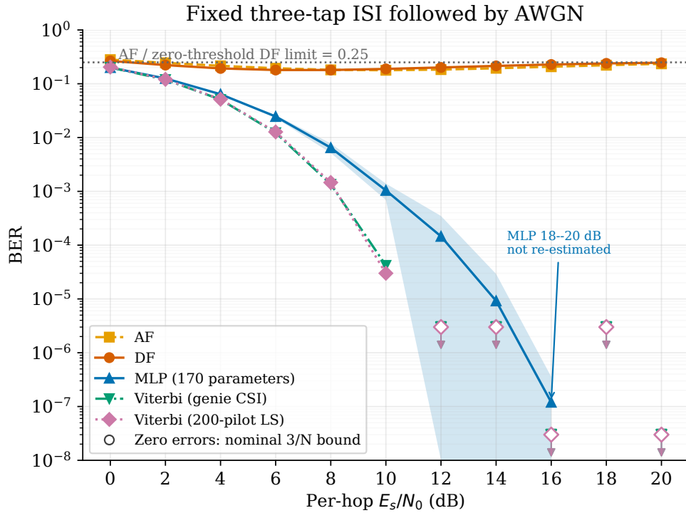
Figure 6.2: Destination BER versus per-hop E_s/N_0 . The original figure is regenerated with the same matched Viterbi sources as Table 6.3. MLP points above 16 dB are omitted. Open Viterbi markers show zero-error nominal 3/N bounds at the actual bit budgets, with downward arrows; these are not measured BERs. AF/DF/MLP bands use the stored across-checkpoint uncertainty at 12–16 dB and the historical intervals below 12 dB
