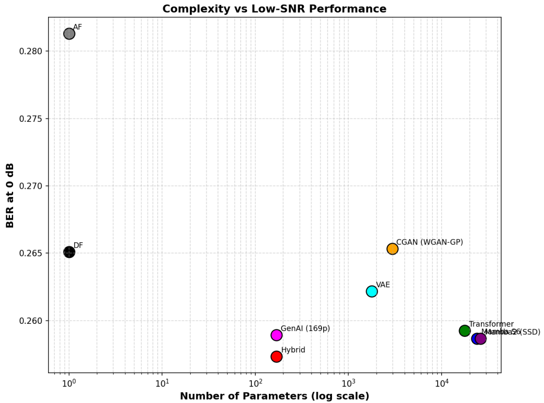
Figure 5.2: Complexity versus low-SNR performance. BER at 0 dB is shown as a function of model size.
