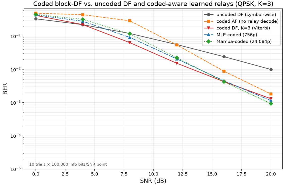
Figure 5.4: The data of Table 5.5 plotted: coded block-DF crosses below uncoded symbol-wise DF between 4 and 8 dB and stays below it thereafter; coded AF, which never decodes, never catches up. Both coded-aware learned relays track coded-DF closely from 12 dB up but are visibly worse at 4–8 dB.
