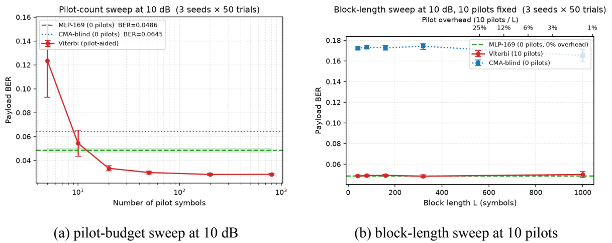
Figure 6.5: Partial-posterior regime; both panels are means over 50 channel draws at 20,000 bits/-point. (a) Pilot-aided Viterbi outperforms the pilot-free MLP down to approximately 20 pilots per block, loses its edge by 10 pilots, and collapses at 5 pilots when the least-squares estimate becomes too noisy to construct a reliable trellis ( 0.1235 \pm 0.0304 ); the MLP is flat across the sweep, operating with an amortized posterior and requiring no pilots. (b) With 10 pilots per block, pilot-aided Viterbi and the MLP are indistinguishable in payload BER at every block length (both \approx 0.049 ), but the classical receiver’s pilot overhead grows from approximately 1% at L = 1000 to 25% at L = 40 . Blind CMA, the other pilot-free option, cannot converge within blocks this short and sits roughly three and a half times worse throughout. The MLP therefore matches the pilot-aided receiver’s reliability at no overhead, and is the only pilot-free method that stays reliable for short packets
