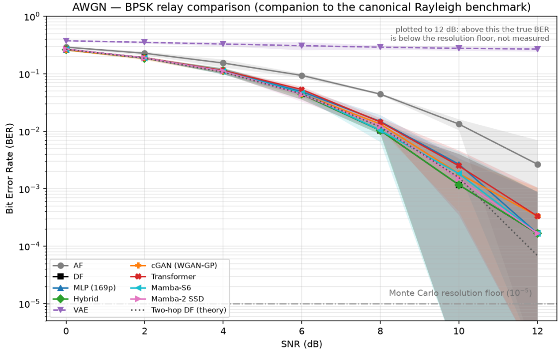
Figure 5.5: AWGN channel: BER vs. SNR for all nine relay strategies with 95% CI, companion to Figure 5.4 and Table 5.5. Plotted only to 12 dB. The dash-dotted line marks the 10^{-5} Monte Carlo resolution floor set by the 100,000-bit budget per SNR point; beyond 12 dB the true AWGN BER falls below it (analytically 2.8 \times 10^{-10} at 16 dB), so points there would trace the floor rather than the relays. The dotted grey curve is the closed-form two-hop DF BER, which the measured curves track.
