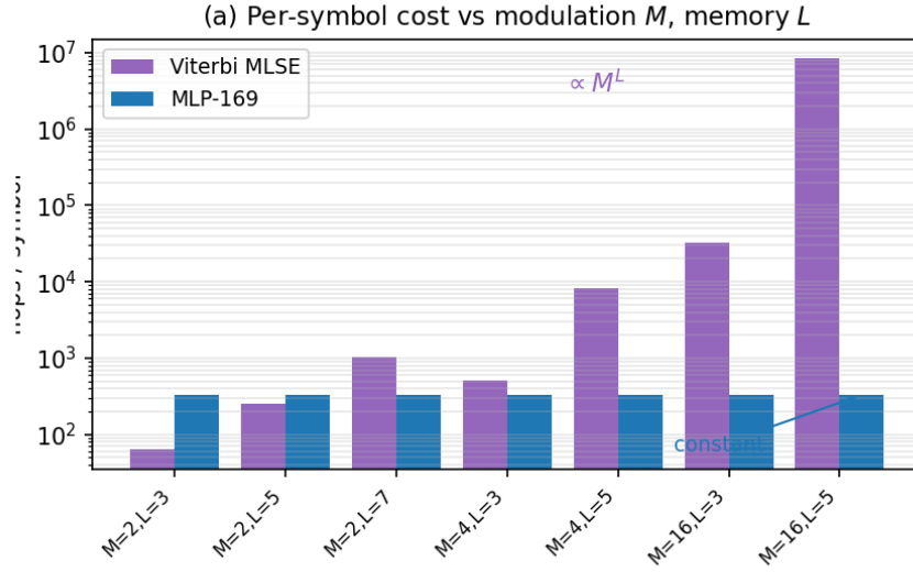
Figure 6.7: Per-symbol computational cost versus modulation order M and channel memory L . Per-symbol operations: Viterbi grows as M^L (intractable by M=16 , L=5 ), while the network grows only linearly in window length and output dimension ( \sim 330 flops for the deployed BPSK, L=3 relay). On the small studied channel (BPSK, L=3 ) Viterbi is actually cheaper; the MLP wins on scaling , not on the small case.
