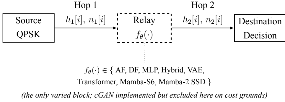
Figure 1.1: Canonical two-hop relay benchmark used throughout the thesis. The source, the channel model on both hops, and the destination are the same in every experiment of the canonical comparison; only the relay processing function f_{\theta}(\cdot) (dashed) is varied among the eight candidate strategies compared there. The fading itself is not static: h_1[i] and h_2[i] are redrawn every symbol. Observed BER differences in the canonical comparison are therefore attributable to the relay strategy alone.
