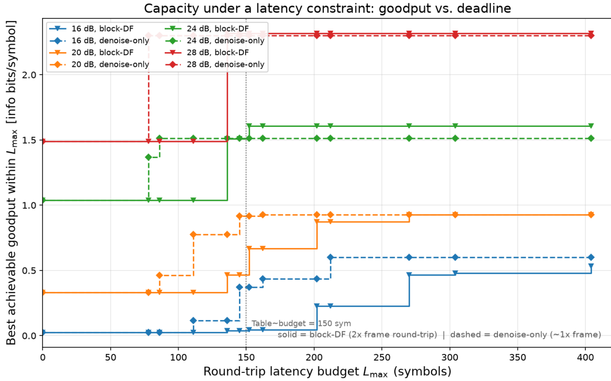
Figure 5.5: Best achievable goodput as a function of the idealized buffer-readiness budget L_{\max} , at the four SNRs where the two relay strategies differ (16, 20, 24, 28 dB). Each curve is a step function under this accounting. The omitted two-hop transmission time prevents interpreting this axis as end-to-end latency
