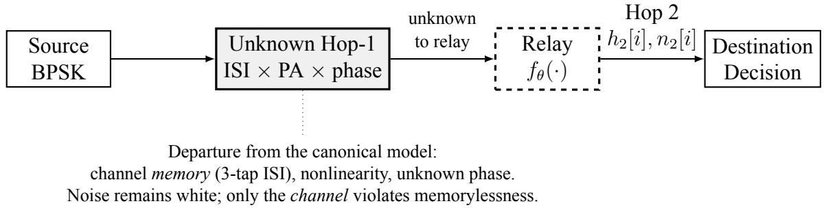
Figure 6.1: Unknown/mismatched-channel study (Chapter 6), a deliberate departure from the canonical benchmark of Figure 1.1. The Hop-1 channel is replaced by an unknown impairment (3-tap ISI, amplifier nonlinearity, and unknown phase) that is not disclosed to any relay. The noise remains white; only the channel violates the memoryless assumption, which is why sequence detection (Viterbi MLSE) becomes the relevant classical benchmark here and nowhere else in the thesis
