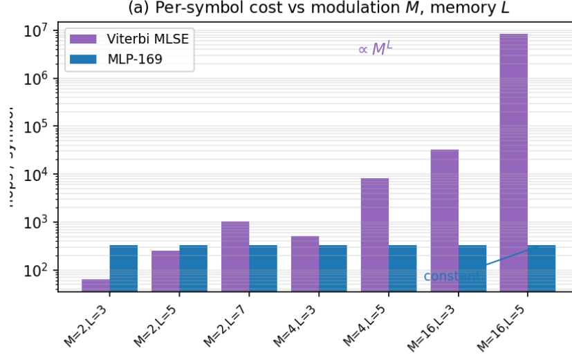
Figure 6.7: Per-symbol computational cost versus modulation order M and channel memory L . Per-symbol operations: Viterbi grows as M^L (intractable by M=16, L=5 ), while the network grows only linearly in window length and output dimension ( \sim 330 flops for the deployed BPSK, L=3 relay). On the small studied channel (BPSK, L=3 ) Viterbi is actually cheaper; the MLP wins on scaling , not on the small case
