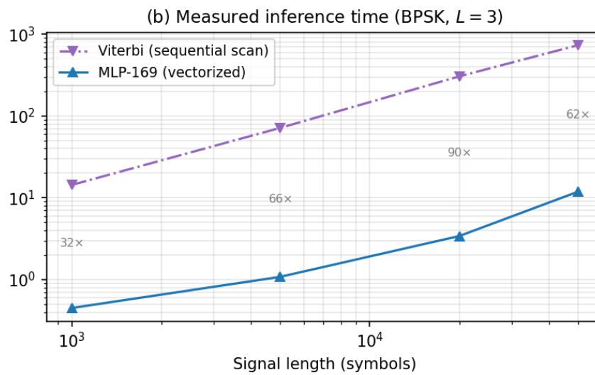
Figure 6.8: Measured inference time for BPSK with L = 3 : the MLP is 30–90× faster as a vectorized matmul versus Viterbi’s interpreted sequential trellis scan
