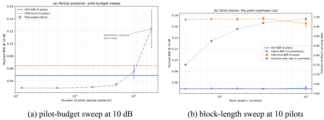
Figure 6.5: Partial-posterior regime; both panels are means over 50 channel draws at 20,000 bits/point. (a) Pilot-aided Viterbi outperforms the pilot-free MLP down to approximately 20 pilots per block, loses its edge by 10 pilots, and collapses at 5 pilots when the least-squares estimate becomes too noisy to construct a reliable trellis ( 0.1235 \pm 0.0304 ); the MLP is flat across the sweep, operating with an amortized posterior and requiring no pilots. (b) With 10 pilots per block, pilot-aided Viterbi and the MLP are indistinguishable in payload BER at every block length (both \approx 0.049 ), but the classical receiver’s pilot overhead grows from approximately 1% at L = 1000 to 25% at L = 40 . Blind CMA, the other pilot-free option, cannot converge within blocks this short and sits roughly three and a half times worse throughput. The MLP therefore matches the pilot-aided receiver’s reliability at no overhead, and is the only pilot-free method that stays reliable for short packets
