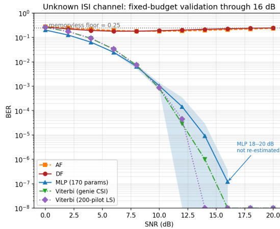
Figure 6.2: Unknown-channel relaying, BER vs. SNR. Historical 0–10 dB values are retained; the 12–16 dB AF, DF, and MLP points and their 95% across-checkpoint t bands are replaced by predeclared fixed-budget measurements (three checkpoints; 10M bits/checkpoint at 12–14 dB and 100M at 16 dB). The MLP’s 18–20 dB historical rare-event tail is intentionally omitted pending validation. AF/DF remain near the analytic 0.25 floor; the MLP falls sharply through the validated range, while genie-CSI Viterbi and 200-pilot LS MLSE provide the model-aware reference
