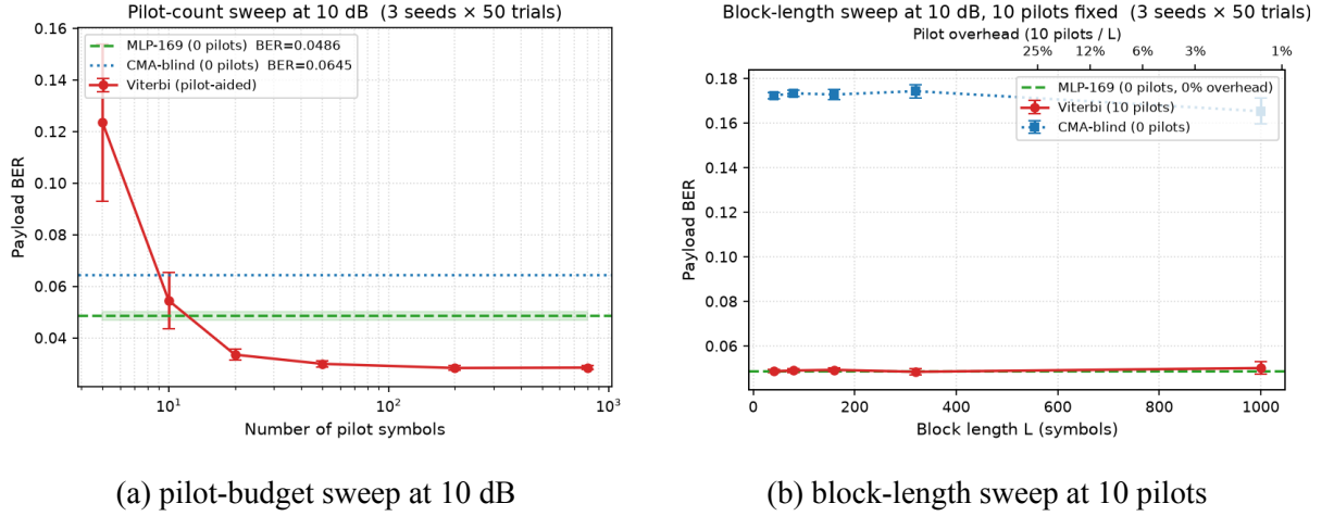
Figure 6.5: Finite-pilot regime; both panels are means over 50 channel draws at 20,000 bits/point. (a) Pilot-aided Viterbi outperforms the pilot-free MLP down to approximately 20 pilots per block, loses its edge by 10 pilots, and collapses at 5 pilots when the least-squares estimate becomes too noisy to construct a reliable trellis ( 0.1235 \pm 0.0304 ); the MLP is flat across the sweep, operating with a family-trained discriminative estimator and requiring no pilots. (b) With 10 pilots per block, pilot-aided Viterbi and the MLP have no detected payload-BER difference at the evaluated block lengths (both \approx 0.049 ), but the classical receiver’s pilot overhead grows from approximately 1% at L = 1000 to 25% at L = 40 . Blind CMA, the other pilot-free option, cannot converge within blocks this short and sits roughly three and a half times worse throughout. The MLP therefore matches the pilot-aided receiver’s reliability at no overhead, and is the only pilot-free method that stays reliable for short packets
