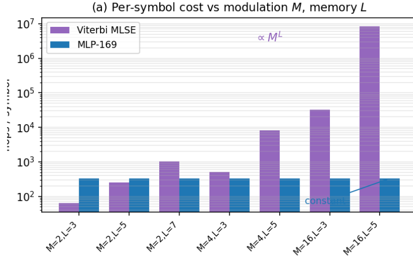
Figure 7.8: Per-symbol computational cost versus modulation order M and channel memory L . Per-symbol operations: Viterbi grows as M^L (intractable by M=16 , L=5 ), while the network grows only linearly in window length and output dimension ( \sim 330 flops for the deployed BPSK, L=3 relay). On the small studied channel (BPSK, L=3 ) Viterbi is actually cheaper; the MLP wins on scaling , not on the small case.
