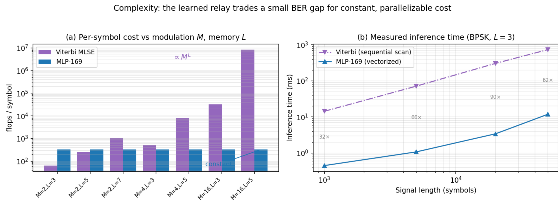
Figure 7.5: Complexity of Viterbi MLSE vs the 170-parameter MLP. (a) Per-symbol operations: Viterbi grows as M^L (intractable by M=16 , L=5 ), while the MLP is constant at \sim 330 flops. On the small studied channel (BPSK, L=3 ) Viterbi is actually cheaper; the MLP wins on scaling , not on the small case. (b) Measured inference time (reference implementations): the MLP is 30\text{--}90\times faster as a vectorized matmul versus Viterbi’s interpreted sequential trellis scan.
