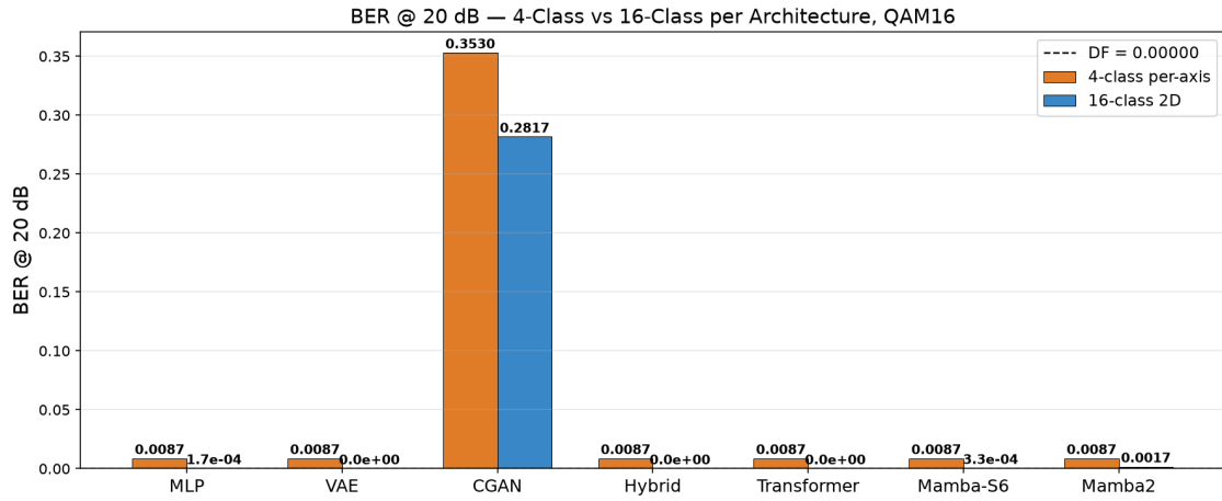
Figure 6.8: Grouped bar comparison of 4-class vs. 16-class BER at 20 dB for each architecture. The joint 16-class formulation drives the BER to (near-)zero for every architecture except the CGAN, which fails to converge in both formulations (0.353 / 0.282) and dominates the plot at this scale.
