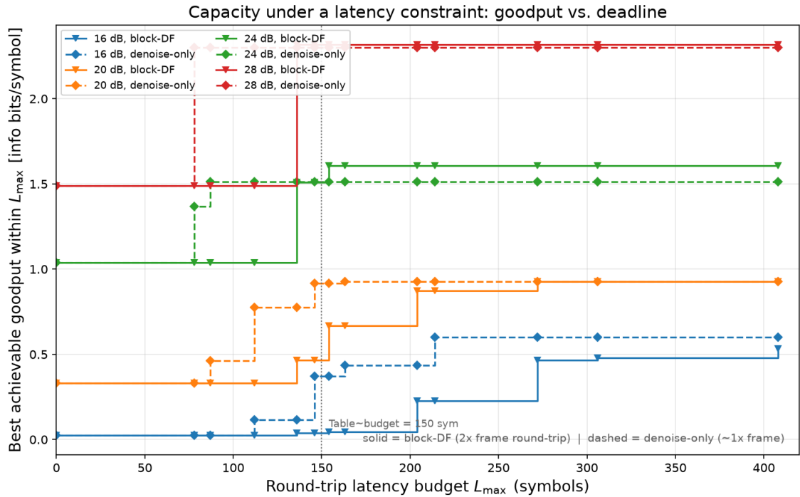
Figure 5.12: Best achievable goodput as a function of the round-trip latency budget L_{\max} , at the four SNRs where the two relay strategies differ (16, 20, 24, 28 dB). Each curve is a step function: goodput jumps each time L_{\max} crosses an MCS’s round-trip latency. The denoise-only relay’s steps (dashed) occur at roughly half the L_{\max} of the block-DF relay’s (solid) for a comparable rate, since block-DF pays the frame cost twice.
