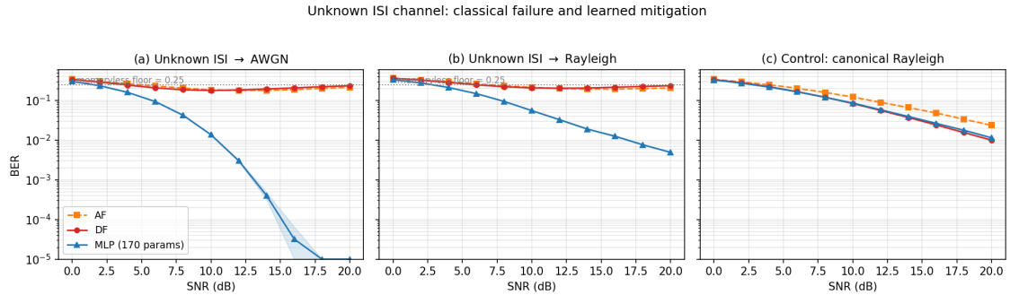
Figure 7.1: Unknown-channel relaying, BER vs. SNR with 95% CI bands. (a)–(b) On the unknown ISI channel, the memoryless AF/DF relays are pinned near the analytic 0.25 floor (DF non-monotonic in SNR); the 170-parameter MLP restores monotonically decreasing BER within \approx 1 – 1.5 dB of genie-CSI Viterbi MLSE, which a 200-pilot LS estimate matches almost exactly. With the Rayleigh second hop (b), MLSE and the MLP are statistically indistinguishable end-to-end. (c) Control: on the canonical Rayleigh channel the MLP only matches DF, consistent with H2.
