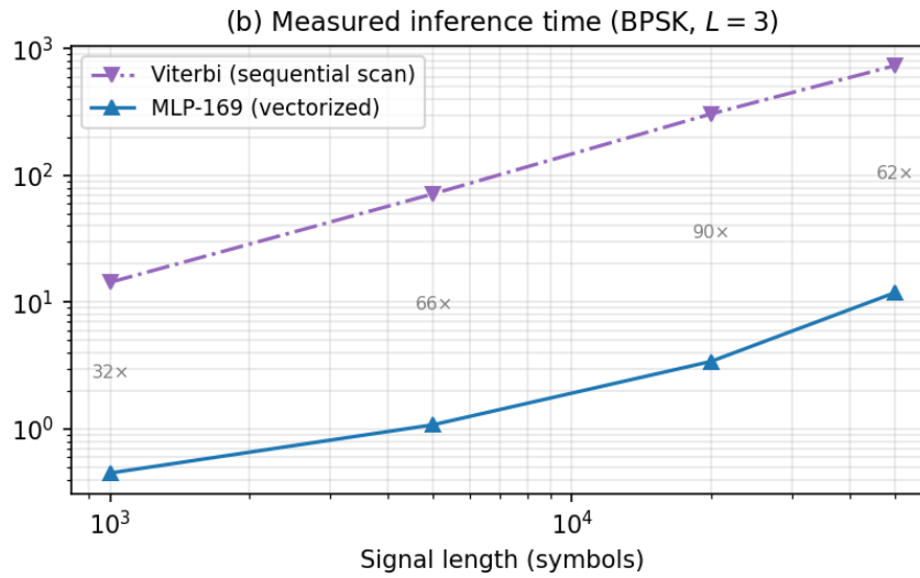
Figure 7.8: Measured inference time for BPSK with L = 3 : the MLP is 30–90 \times faster as a vectorized matmul versus Viterbi’s interpreted sequential trellis scan.
