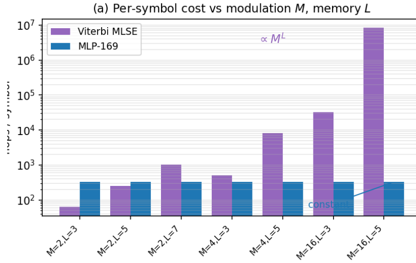
Figure 7.7: Per-symbol computational cost versus modulation order M and channel memory L . Per-symbol operations: Viterbi grows as M^L (intractable by M=16, L=5 ), while the MLP is constant at \sim 330 flops. On the small studied channel (BPSK, L=3 ) Viterbi is actually cheaper; the MLP wins on scaling , not on the small case.
