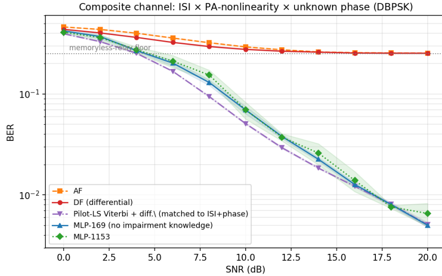
Figure 7.3: Composite channel (ISI \times PA-nonlinearity \times unknown phase, DBPSK). Naive classical relays (AF, differential detection) saturate at the memoryless-relay floor; the 169-parameter MLP restores reliable relaying from raw I/Q with no impairment model, tracking about 2 dB behind the strongest constructed classical baseline (pilot-LS Viterbi + differential). The 1,153-parameter MLP adds nothing (H3).
