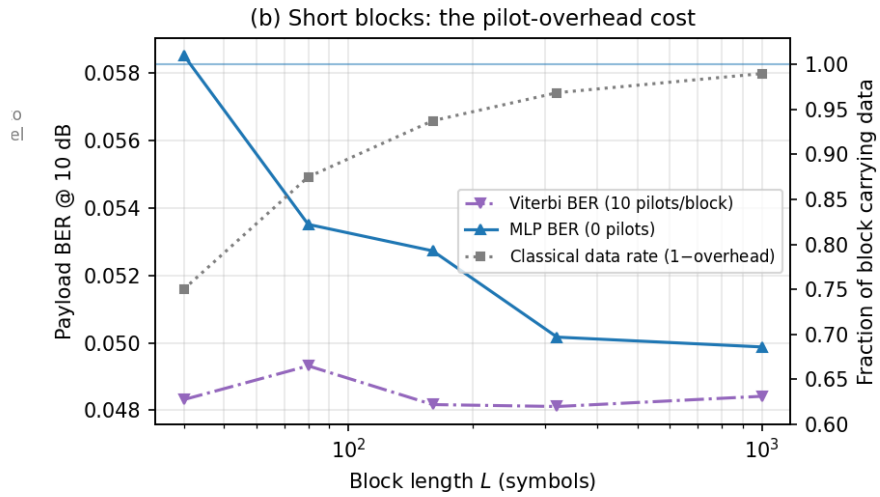
Figure 7.6: Block-length sweep with 10 pilots per block. Payload BER remains similar across methods, but the effective pilot overhead of the classical approach increases rapidly as the block length decreases, growing from approximately 1% at L = 1000 to 25% at L = 40 . The pilot-free MLP incurs no such overhead and therefore becomes increasingly attractive for short packets.
