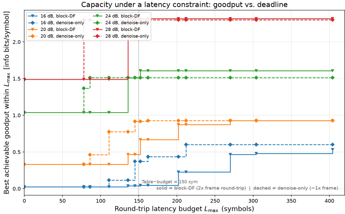
Figure 5.10: Best achievable goodput as a function of the round-trip latency budget L_{\max} , at the four SNRs where the two relay strategies differ (16, 20, 24, 28 dB). Each curve is a step function: goodput jumps each time L_{\max} crosses an MCS’s round-trip latency. The denoise-only relay’s steps (dashed) occur at roughly half the L_{\max} of the block-DF relay’s (solid) for a comparable rate, since block-DF pays the frame cost twice
