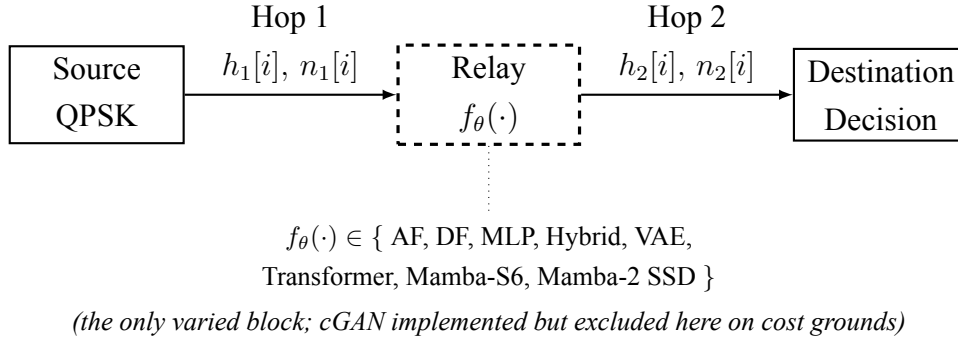
Figure 1.1: Canonical two-hop relay benchmark used throughout the thesis. The source, the channel model on both hops, and the destination are the same in every experiment of the canonical comparison; only the relay processing function f_{\theta}(\cdot) (dashed) is varied among the eight candidate strategies compared there. The fading itself is not static: h_1[i] and h_2[i] are redrawn every symbol. Observed BER differences in the canonical comparison are therefore attributable to the relay strategy alone
