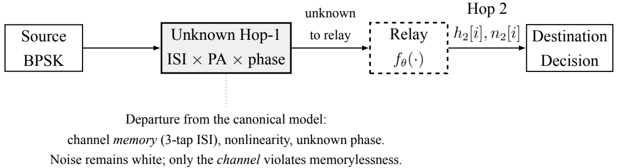
Figure 6.1: Unknown/mismatched-channel study (Chapter 6), a deliberate departure from the canonical benchmark of Figure 1.1. The Hop-1 channel is replaced by an unknown impairment (3-tap ISI, amplifier nonlinearity, and unknown phase) that is not disclosed to any relay. The noise remains white; only the channel violates the memoryless assumption, which is why sequence detection (Viterbi MLSE) becomes the relevant classical benchmark here and nowhere else in the thesis
