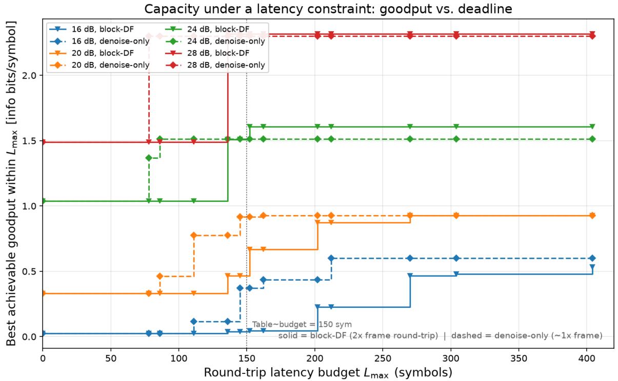
Figure 5.8: Best achievable goodput as a function of the round-trip latency budget L_{\max} , at the four SNRs where the two relay strategies differ (16, 20, 24, 28 dB). Each curve is a step function: goodput jumps each time L_{\max} crosses an MCS’s round-trip latency. The denoise-only relay’s steps (dashed) occur at roughly half the L_{\max} of the block-DF relay’s (solid) for a comparable rate, since block-DF pays the frame cost twice
