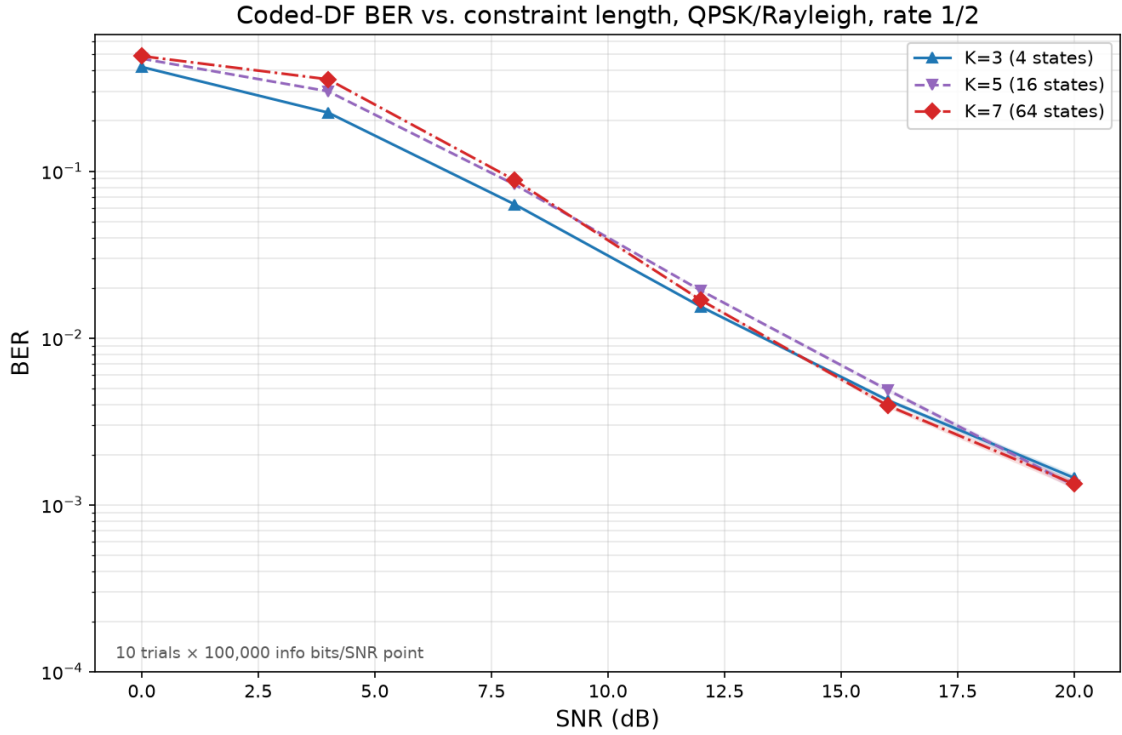
Figure 5.8: The data of Table 5.8 plotted: K=5 and K=7 sit visibly above K=3 at 0–8 dB and only draw level by 16–20 dB, never separating out cleanly ahead of it within this SNR range.
