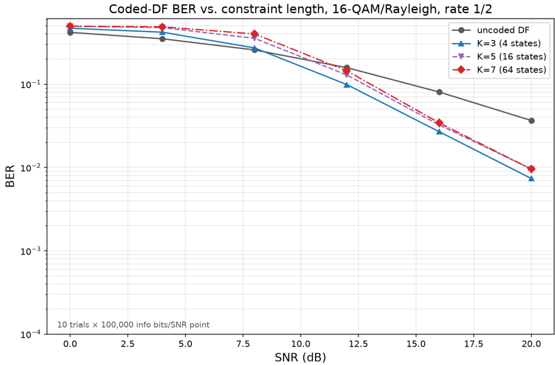
Figure 5.9: The data of Table 5.9 plotted: the same ordering as QPSK, with the coded/uncoded crossover pushed out to roughly 8–12 dB by 16-QAM’s higher baseline uncoded BER, and K=3 remaining the best of the three constraint lengths at every tabulated point.
