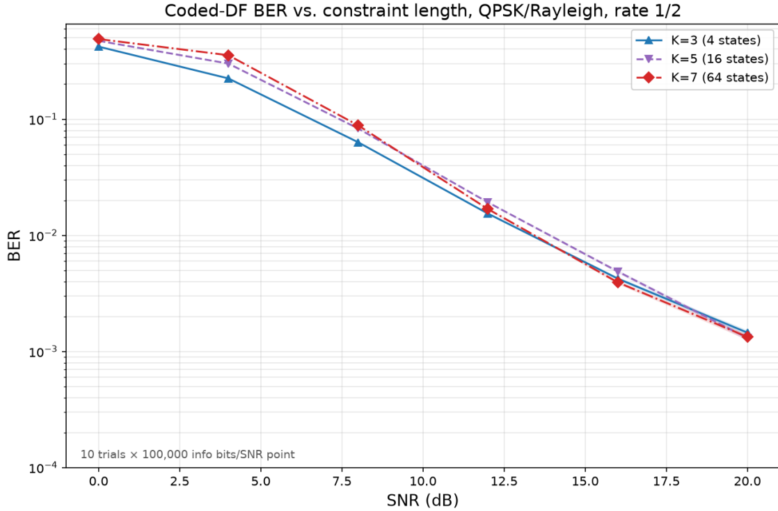
Figure 5.5: The data of Table 5.7 plotted: K=5 and K=7 sit visibly above K=3 at 0–8 dB and only draw level by 16–20 dB, never separating out cleanly ahead of it within this SNR range.
