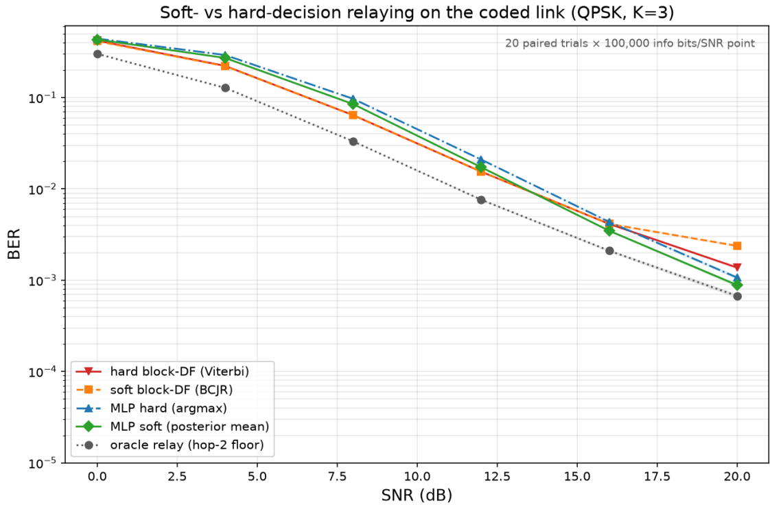
Figure 5.6: The data of Table 5.8. The soft learned relay (green) tracks the oracle floor most closely at high SNR; soft block-DF (orange) turns upward at 20 dB, an artefact of mis-calibration discussed in the text, not of soft forwarding itself.
