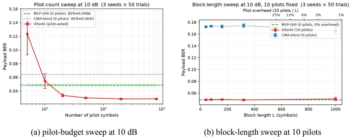
Figure 6.5: Partial-posterior regime; both panels are means over 50 channel draws at 20,000 bits/point. (a) Pilot-aided Viterbi outperforms the pilot-free MLP down to approximately 20 pilots per block, loses its edge by 10 pilots, and collapses at 5 pilots when the least-squares estimate becomes too noisy to construct a reliable trellis ( 0.1235 \pm 0.0304 ); the MLP is flat across the sweep, operating with an amortized posterior and requiring no pilots. (b) With 10 pilots per block, pilot-aided Viterbi and the MLP are indistinguishable in payload BER at every block length (both \approx 0.049 ), but the classical receiver’s pilot overhead grows from approximately 1% at L = 1000 to 25% at L = 40 . Blind CMA, the other pilot-free option, cannot converge within blocks this short and sits roughly three and a half times worse throughout. The MLP therefore matches the pilot-aided receiver’s reliability at no overhead, and is the only pilot-free method that stays reliable for short packets
