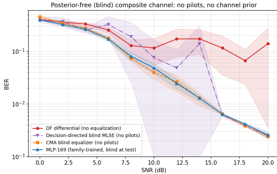
Figure 7.5: Posterior-free composite channel (no pilots, no channel prior, fresh realization per block). CMA (blind classical) and the family-trained MLP converge together; decision-directed blind MLSE is unstable (non-monotonic, wide CI) because it bootstraps the channel from its own decisions; plain differential detection floors. Without a posterior, learning matches, not beats, the best blind classical equalizer, but does so with one-shot, stable inference and no online adaptation.
