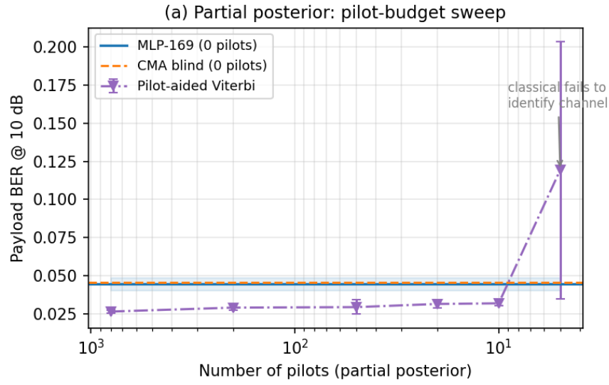
Figure 7.6: Pilot-budget sweep at 10 dB. Pilot-aided Viterbi outperforms the pilot-free MLP down to approximately 10 pilots per block, but collapses at 5 pilots when the least-squares channel estimate becomes too noisy to construct a reliable trellis ( 0.119 \pm 0.084 ). In contrast, the MLP remains essentially unchanged because it operates with an amortized posterior and requires no pilots.
