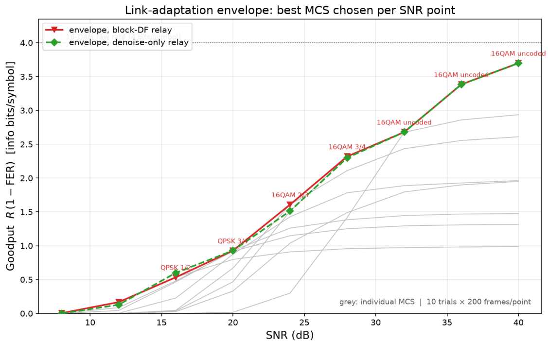
Figure 5.2: The envelope of Table 5.10 (colored) against every individual fixed MCS on the block-DF relay (grey), which is the visual case for adaptation: the envelope tracks the upper hull of the grey curves rather than any single one of them, switching MCS as SNR crosses each rate’s operating threshold. The two relay strategies’ envelopes are visually almost the same curve.
